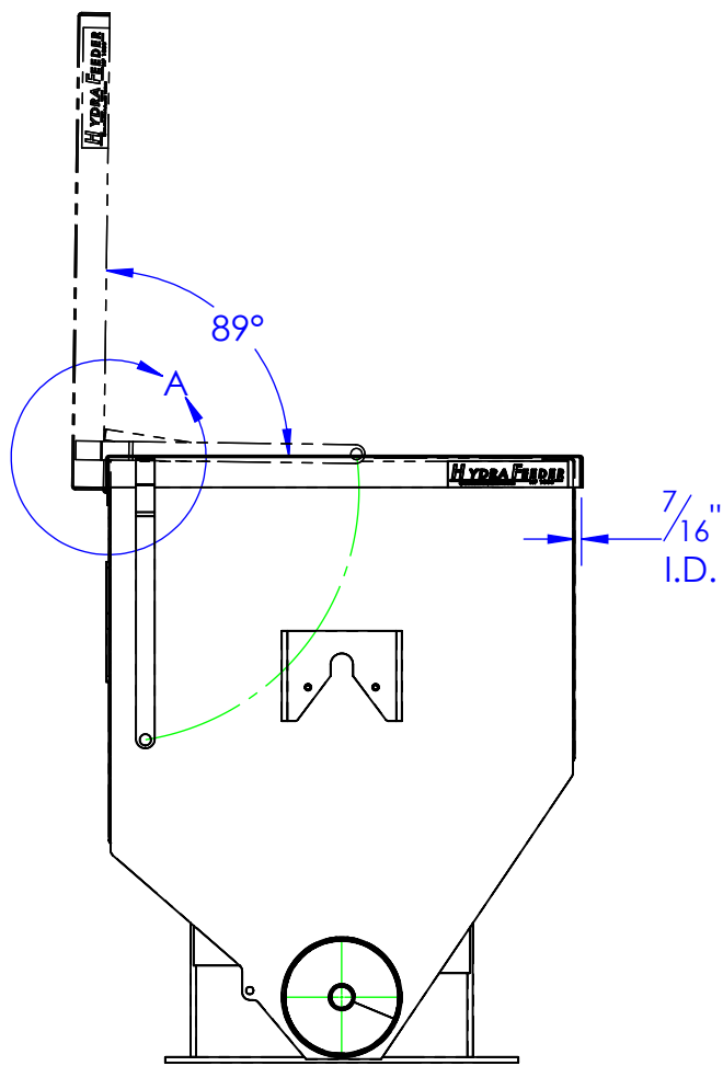
DETAIL A SCALE 1 : 3.5
